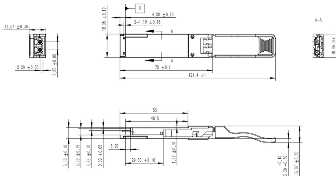
Figure 2. Mechanical dimensions
