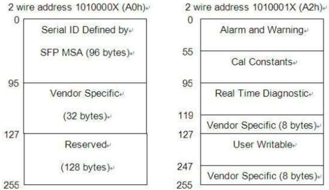
Fig 2 EEPROM Information
